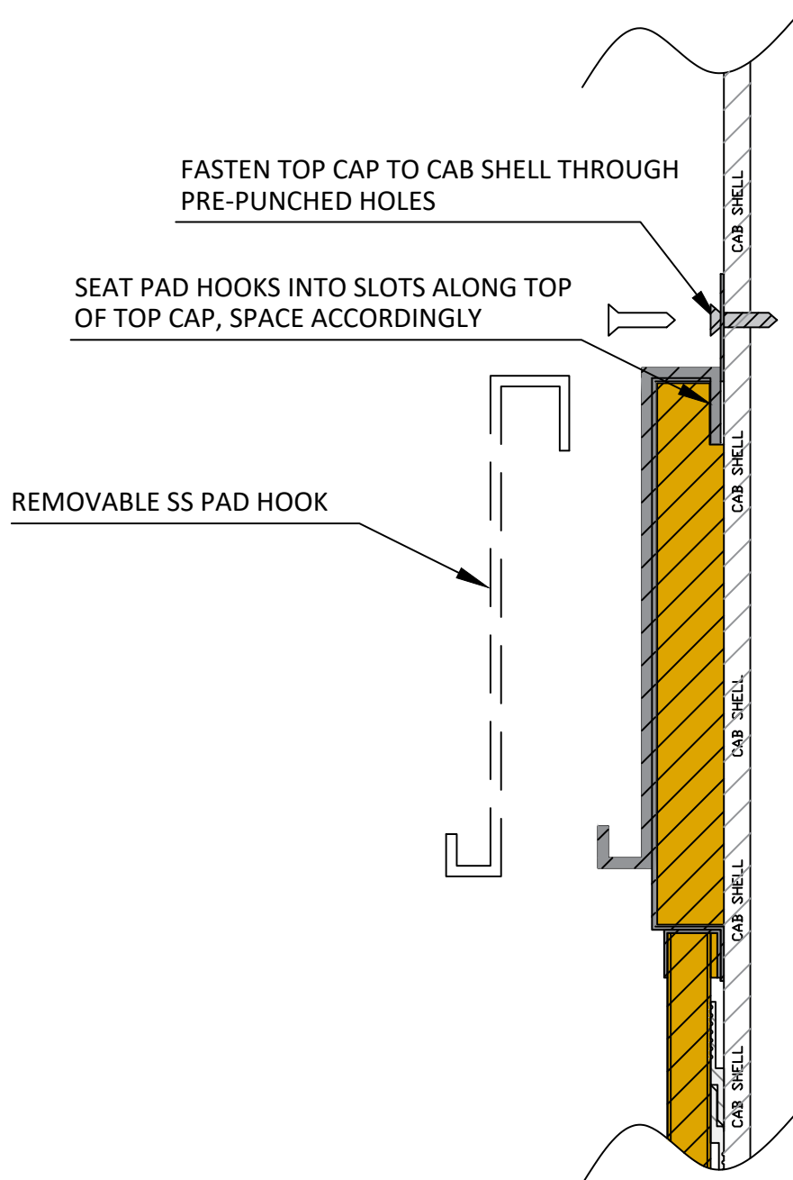
Dia. 13 Top cap detail.
