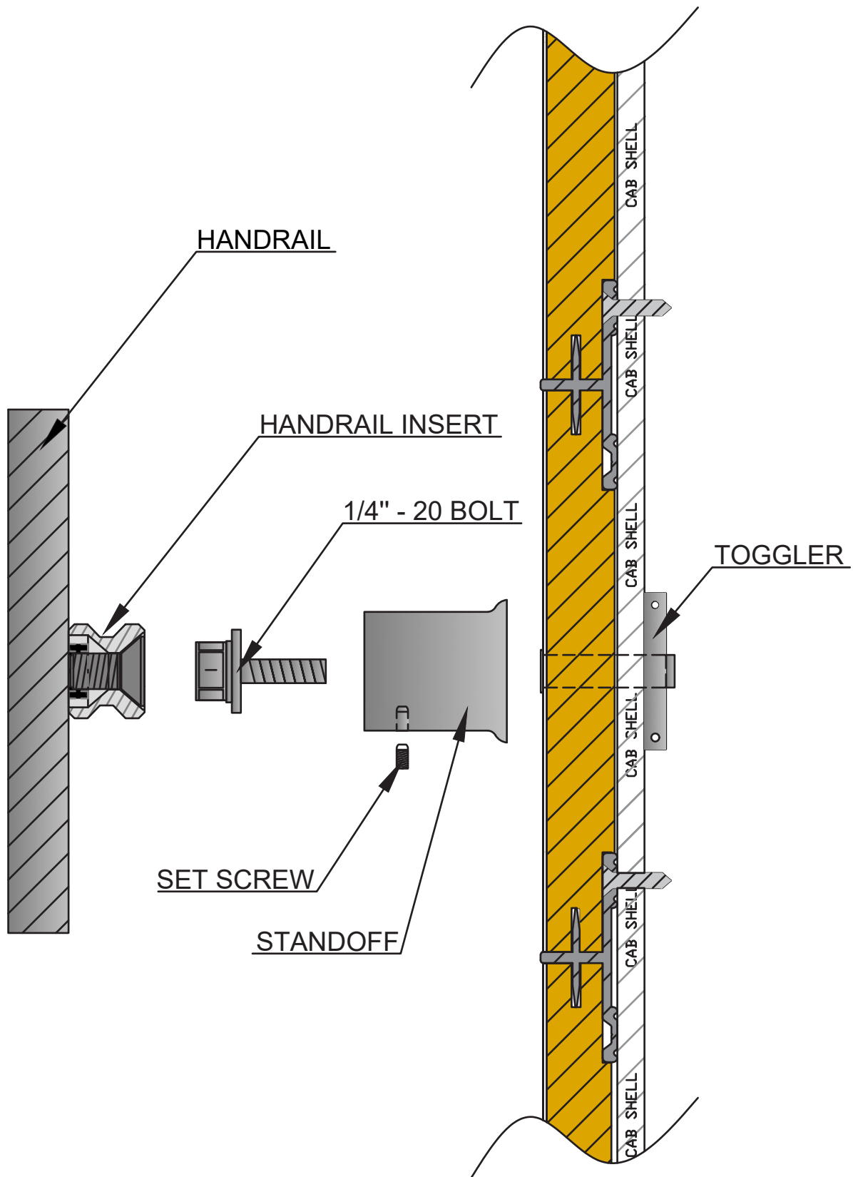
Dia. 8 Attaching standoffs to handrail.
