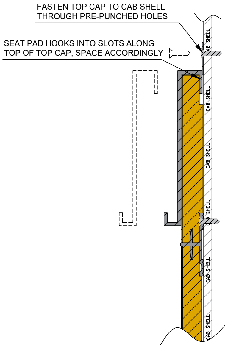
Dia. 13 Top cap detail.
