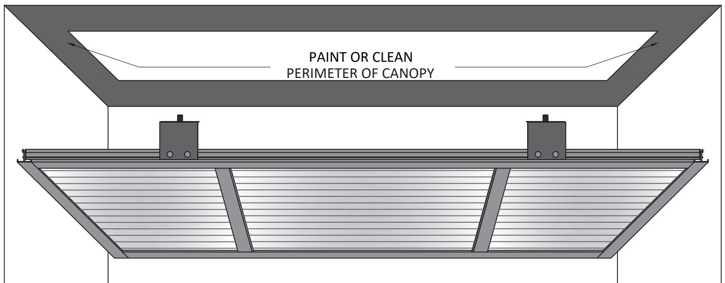
Dia. 1 Framed ceiling preparations.
